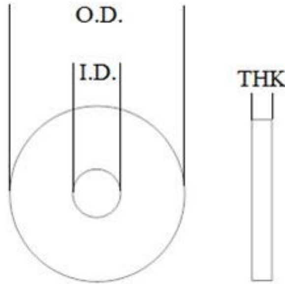
FLAT FENDER WASHERS LOW CARBON STEEL - WEIGHTS & DIMENSIONS
